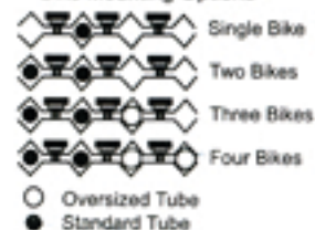
Bike Mounting Options
